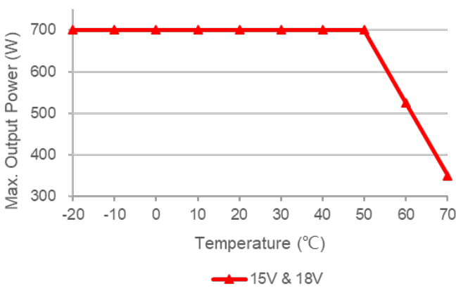
18V Module Max. Output Power Derating Curves
