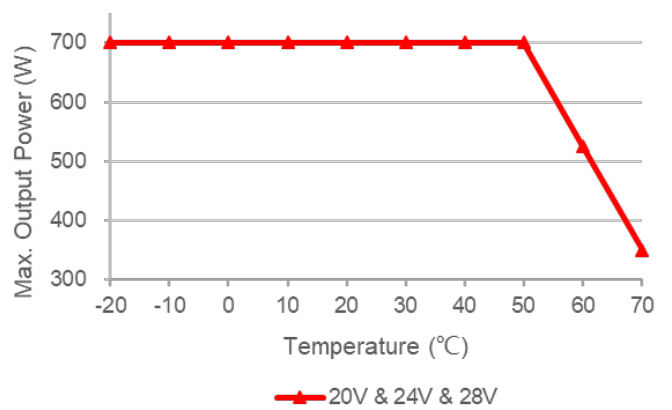
24V Module Max. Output Power Derating Curves
