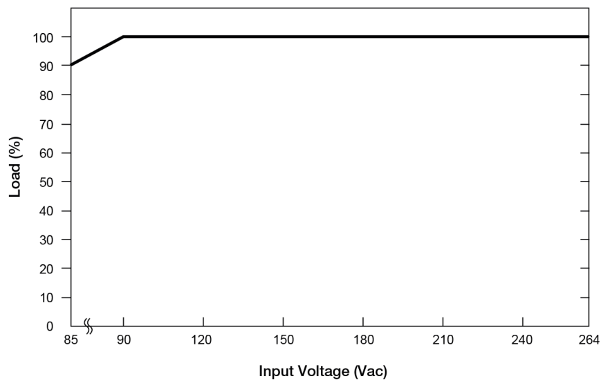
Output Load De-rating VS. Input Voltage
