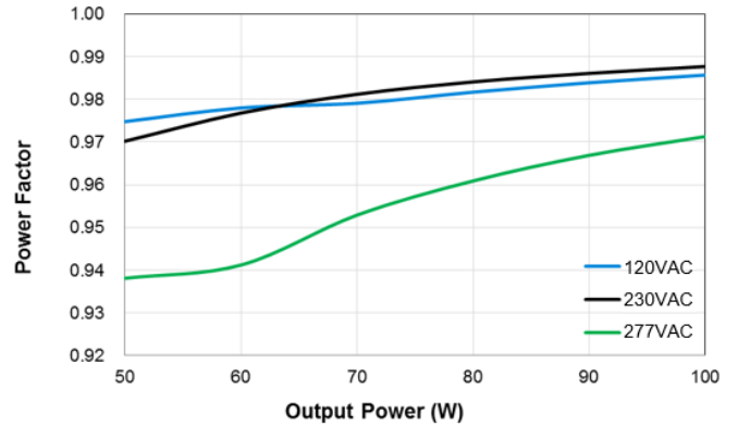
USCO-100140GA – 700mA
