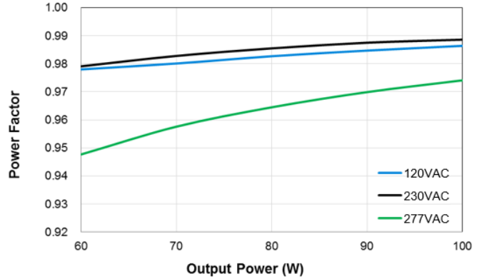
USCO-100140GA – 1400mA
