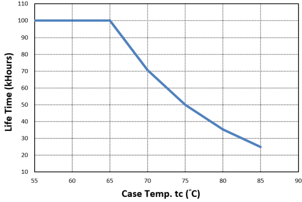
USCO-100140GA
