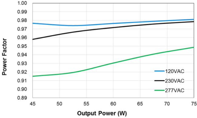
USCO-075140GA – 1400mA
