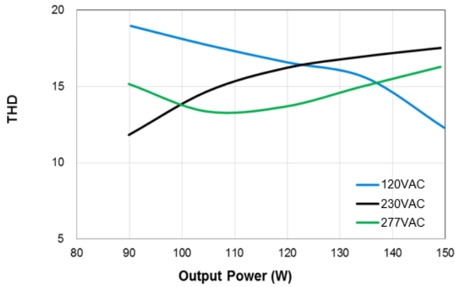
USCO-150140GC – 1400mA
