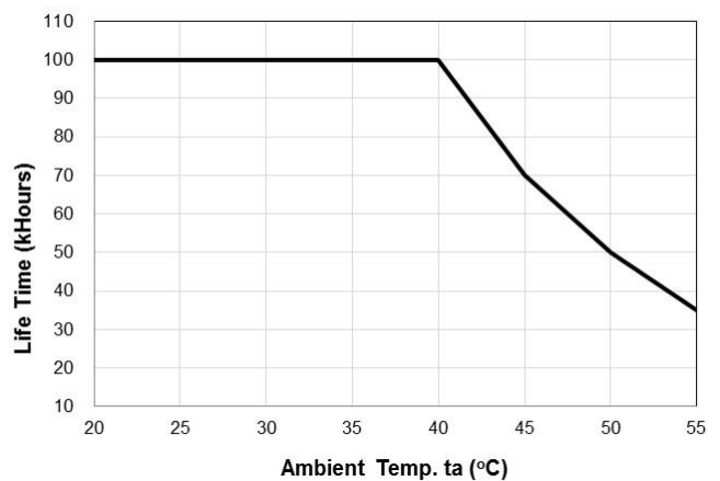
Lifetime VS Ambient Temperature
